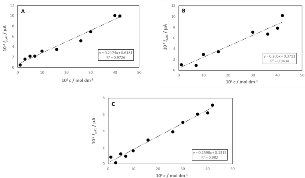
Fig. 5. Anodic peak current of the first oxidation peak ( I_{p,A1} ) of rutin as a function of rutin concentration, scan rate: 5 mV/s. I_c = 0.34 \text{ mol dm}^{-3} KCl (A), NaCl (B) and LiCl (C)
