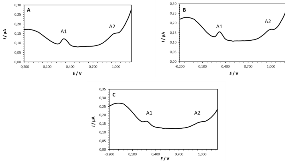
Fig. 4. Differential pulse voltammograms of rutin ( c = 1 \cdot 10^{-5} \text{ mol dm}^{-3} ) recorded at glassy carbon electrode, scan rate: 5 mV/s. I_c = 0.34 \text{ mol dm}^{-3} KCl (A), NaCl (B) and LiCl (C)
