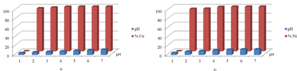
Figure 1. Effect of pH on the efficiency of removing a) \text{Cu}^{2+} and b) \text{Ni}^{2+} from their monocomponent aqueous solutions of initial concentrations 500 mg/L
