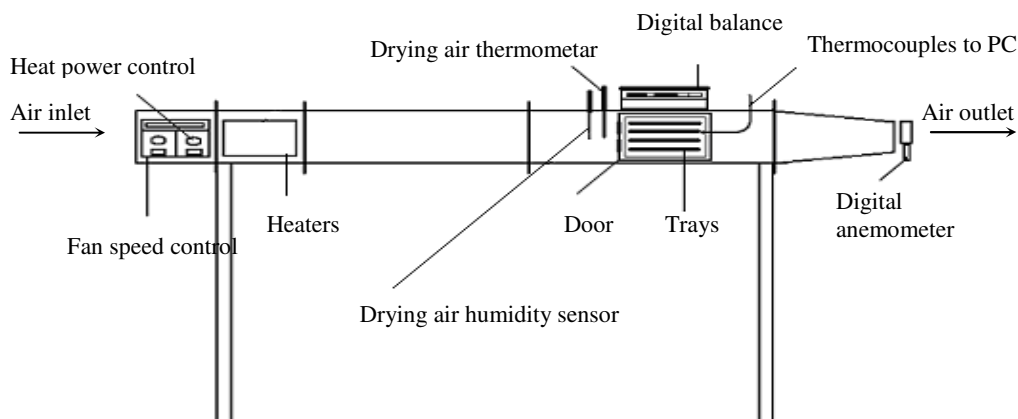
Fig. 1. Laboratory dryer used for convective drying
