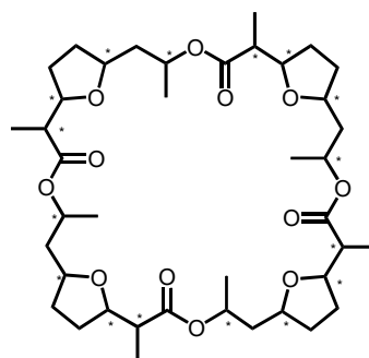
Macrolide: Nonactin
