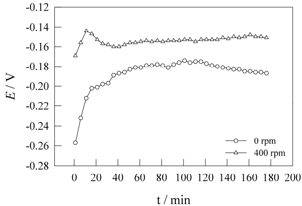
Fig. 1. Variation of open circuit potential with time of the AISI 316L in 0.5 \text{ mol dm}^{-3} NaCl solution at 20 \text{ }^\circ\text{C}
