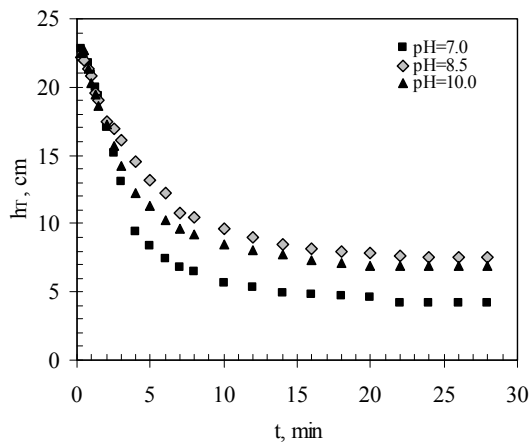
Fig. 2. Settling in suspensions at pH values of 7, 8.5 and 10 without addition of coagulants
