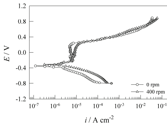
Fig. 2. Potentiodynamic polarization curves of the AISI 316L in 0.5 \text{ mol dm}^{-3} NaCl solution at 20 \text{ }^\circ\text{C}
