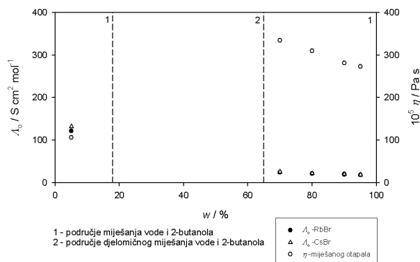
Slika 1. Granična molarna provodnost ( \Lambda_0 ) za RbBr (●) i CsBr (▲) u 5, 70, 80, 90 i 95 mas. %-tnom 2-butanolu pri 25 °C; viskoznost ( \eta ) miješanog otapala pri 25 °C Fig. 1. Molar conductivity ( \Lambda_0 ) of RbBr (●) and CsBr (▲) in 5, 70, 80, 90 and 95 mass. % 2-butanol at 25 °C; viscosity ( \eta ) of 2-butanol + water mixtures
