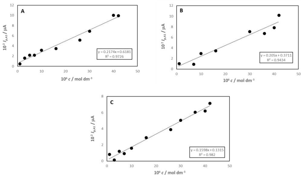
Fig. 5. Anodic peak current of the first oxidation peak ( I_{p,A1} ) of rutin as a function of rutin concentration, scan rate: 5 mV/s. I_c = 0.34 mol \text{dm}^{-3} KCl (A), NaCl (B) and LiCl (C)
