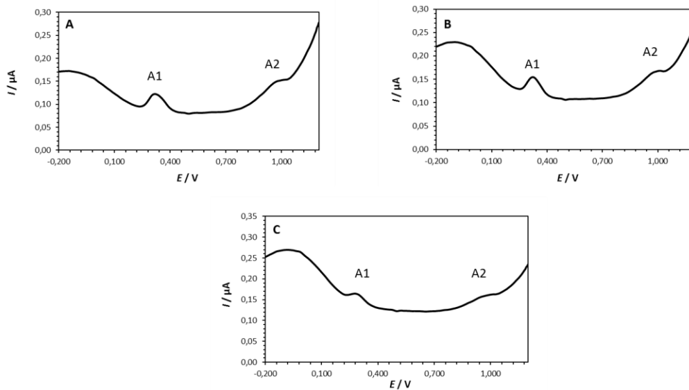
Fig. 4. Differential pulse voltammograms of rutin ( c = 1 \cdot 10^{-5} mol \text{dm}^{-3} ) recorded at glassy carbon electrode, scan rate: 5 mV/s. I_c = 0.34 mol \text{dm}^{-3} KCl (A), NaCl (B) and LiCl (C)
