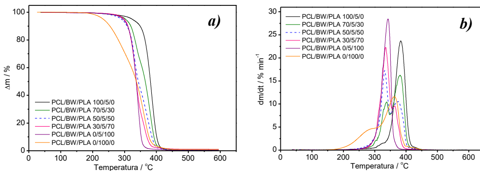
Slika 7. TG (a) i DTG (b) krivulje PCL/BW/PLA mješavina Fig. 7. TG (a) and DTG (b) curves of PCL/BW/PLA blends
