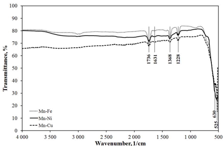
Fig. 6. The FTIR spectrums of the Mn-M (M: Fe, Ni, Cu) mixed oxides
