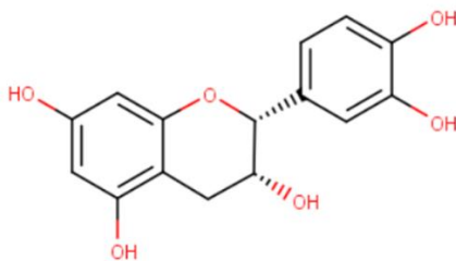
(-)-Epikatehin
