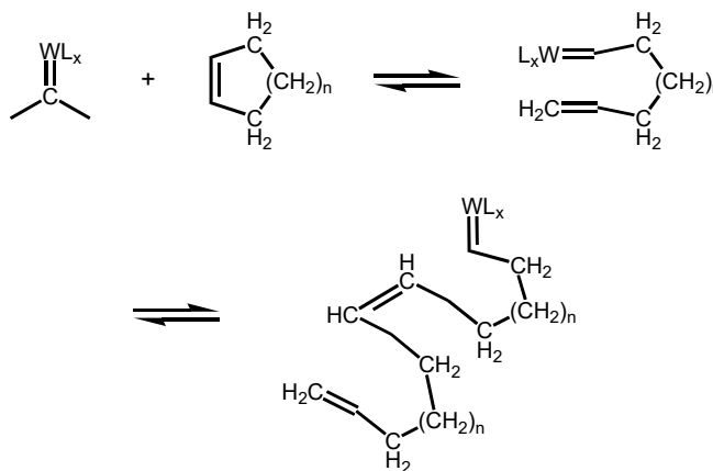
Figure 20. Metathesis polymerization of cyclic olefins.
