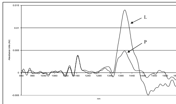
Fig. 3. Samples of the corresponding derivatives of NIR spectra for surimi samples P and L
