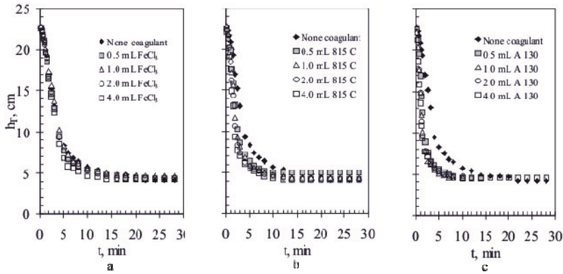
Fig. 3. Graphical dependence of settlement interface against settling time for suspension at pH = 7 with and without coagulants: a) FeCl 3 , b) 815 C, c) A 130
