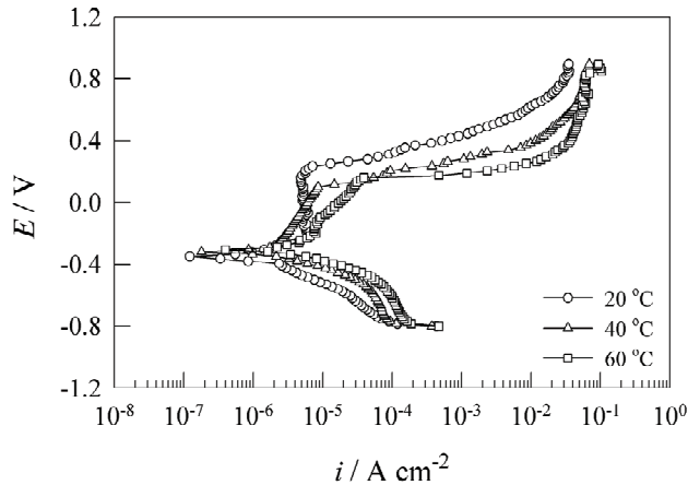
Fig. 3. Potentiodynamic polarization curves of the AISI 316L in quiescent 0.5\text{ mol dm}^{-3} NaCl solution at different temperatures of electrolyte
